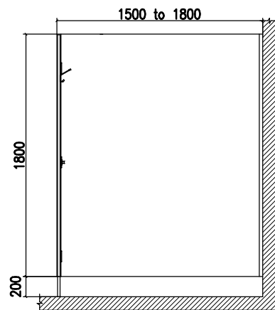
CROSS-SECTION
