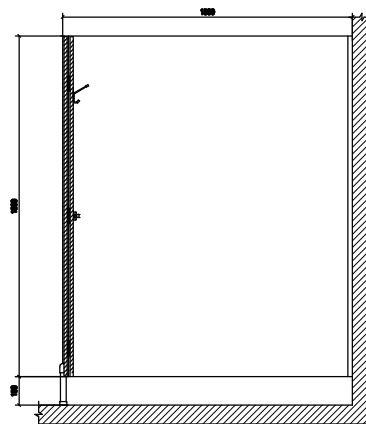
CROSS-SECTION
